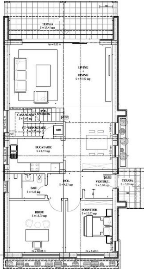
PLAN PARTER
