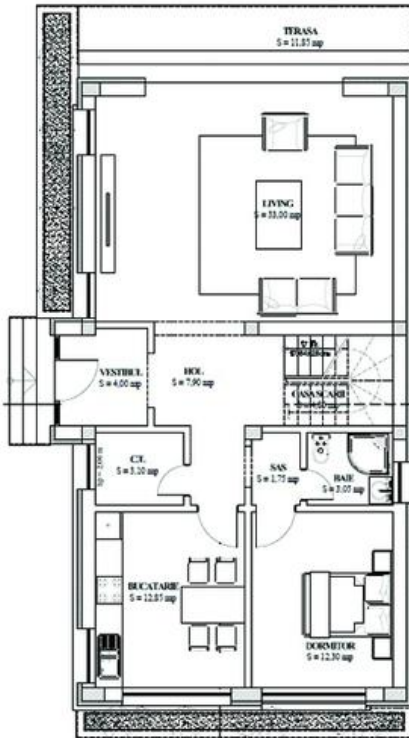
PLAN PARTER
