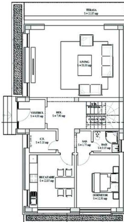
PLAN PARTER
